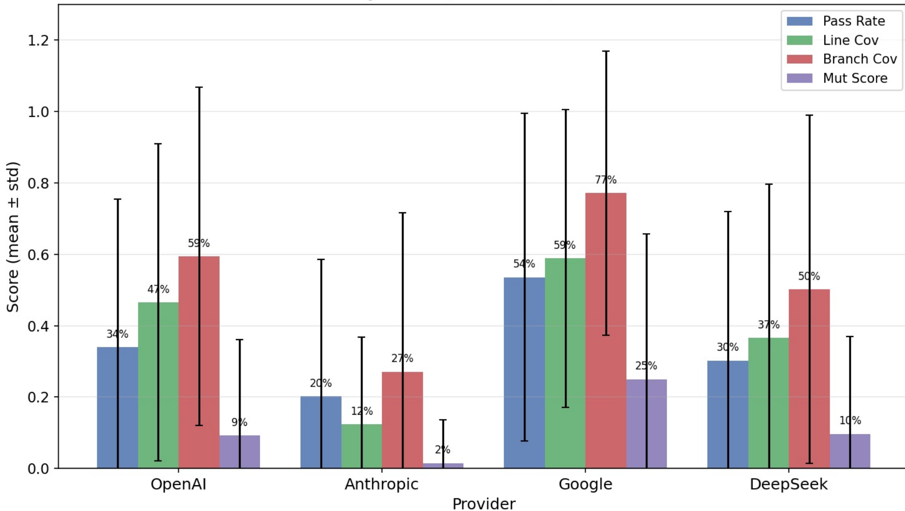
Cross-Provider Comparison (all models, frameworks & k values)
